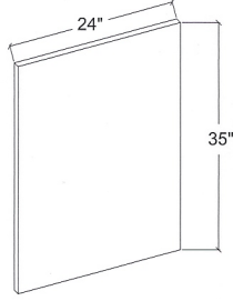
Dishwasher Panel (3/4" thickness) DWP
